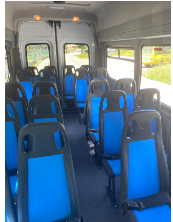
Construction of the passenger seats compliant with DM 01.04.2010 self-extinguishing, vandal-proof with abdominal seat belts, and handle.
